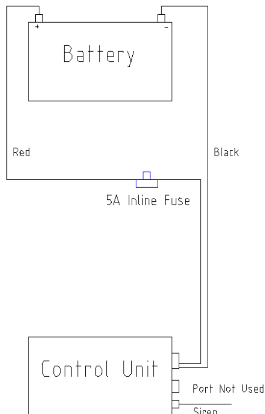
Wiring Diagram
